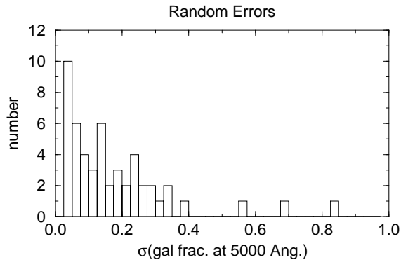
Figure 7. Distribution of 1\sigma random errors in the fractional galaxy contribution at 5000\text{\AA} (rest frame) for Parkes sources. (see section 4.2).
