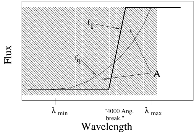
Figure 3. Definition of our “figure of merit” A . For a particular source spectrum f_T(\lambda) (whose 4000Å break region is shown exaggerated), we subtract an amount of galaxy flux, f_g(\lambda) (Fig. 1) until A is a minimum and a smooth power-law f_q(\lambda) results.
