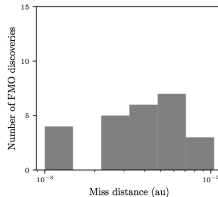
Figure 1: Distribution of miss-distances from Earth for newly discovered Fast Moving Objects from zStreak processing [3].
